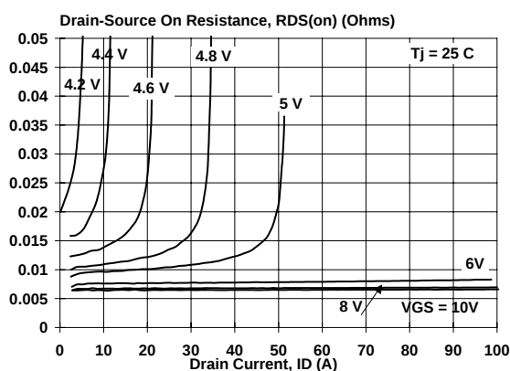
Fig.6. Typical on-state resistance, T_j = 25^\circ\text{C} . R_{DS(ON)} = f(V_{GS})
