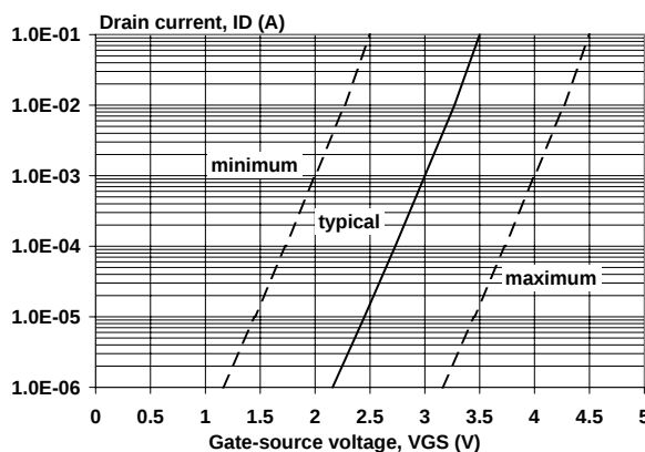
Fig. 11. Sub-threshold drain current. I_D = f(V_{GS}) ; T_j = 25 \text{ °C}
